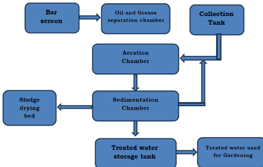
Treatment process involved in 200 KLD and 125 KLD STP installed in the campus
